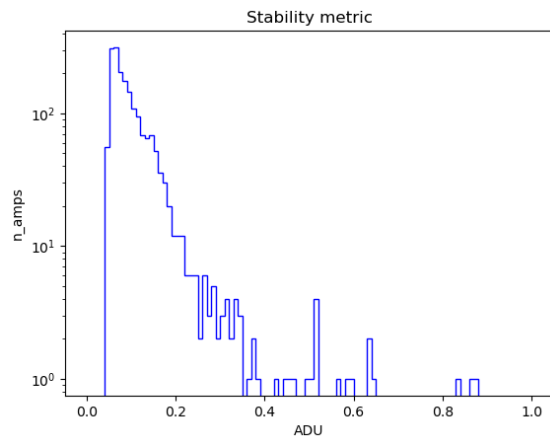
Figure 76: Distribution of the stability metric for the e2v amplifiers in run E2136
