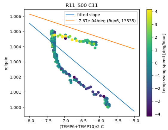
Figure 81: Relative gain as a function of REB temp (TEMP6 and TEMP10), with color based on temperature swing run in run E1367
