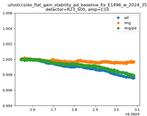
Figure 84: Raw measurements of image count and photodiode integration, as well as the ratio of those – the relative gain for E1496
