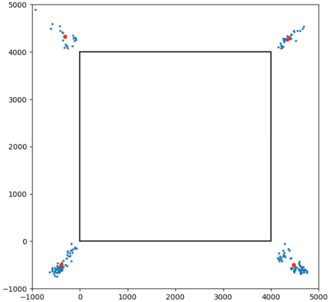
Figure 86: The center of the Tree Rings were measured for all 189 LSST sensors. Red point indicates the average center on each direction.
