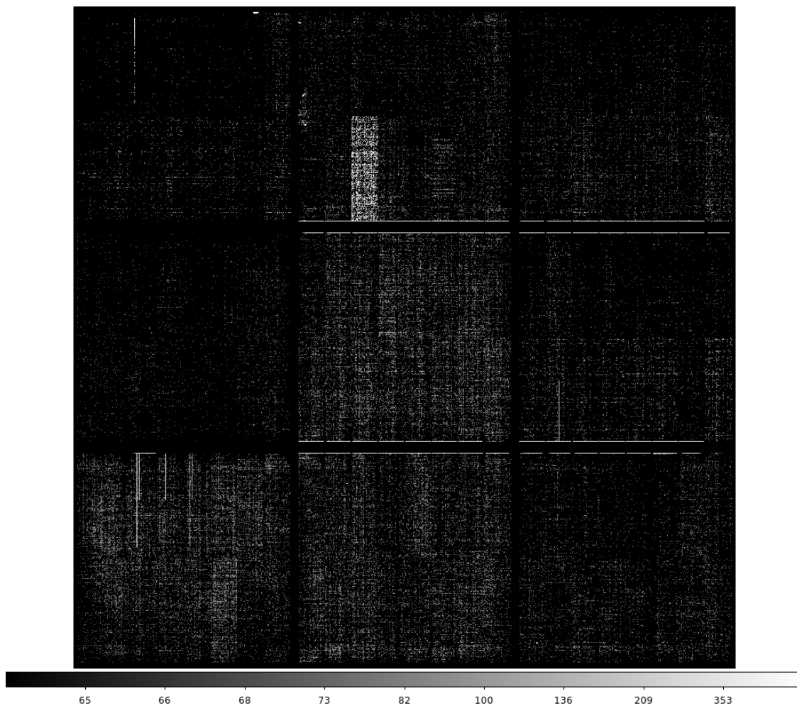
Figure 108: Phosphorescence transients for the R41 RTM captured in the first 15 s following red CCOB LED at 400 ke - /pix. With 8×8 blocking, the upper end of the color scale (640) corresponds to 10 e - /pixel when averaged over 64 pixels contributing.
