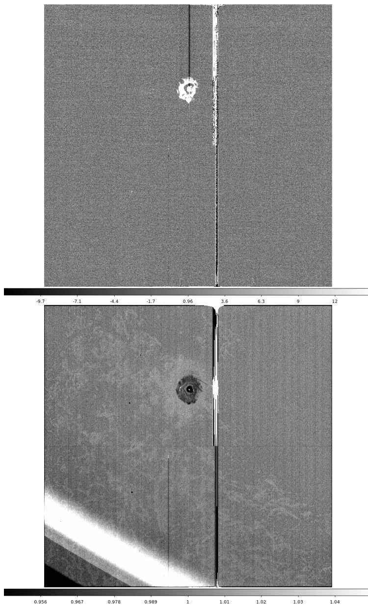
Figure 112: The ITL sensor R01_S00. Top: the transient phosphorescence term. Bottom: the blue flat response. The large, extended spot appears to be centered on a vampire pixel , which also expresses a large amplitude of phosphorescence, which emits enough current to contaminate the parallel overscan in at least the first 15 s exposure following trigger. The flat response feature has opposite polarity from the phosphorescence.
