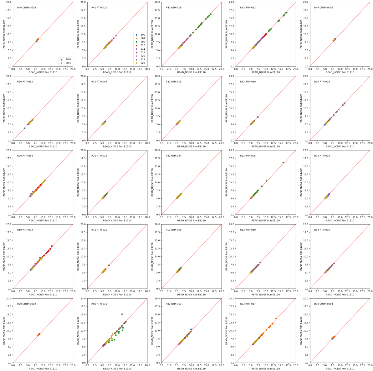
Figure 70: Impact on science sensors read noise from guiders running in guider mode. E1110 has the guider sensors in imaging mode, and E1290 has the guider sensors in guiding mode. The two runs are consistent in read noise.
