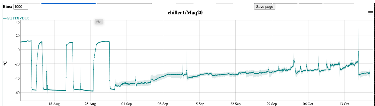
Figure 99: The trend of TXV Bulb temperature at PCS Stage 1, increasing trend showing degradation over time.
