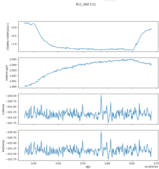
Figure 80: relative gain changes with other parameters for one amplifier R01/S00/C11 in run E1367
