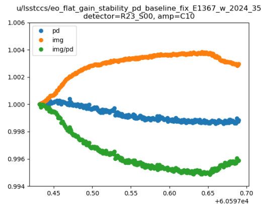
Figure 85: Same as Figure 84 but for E1367
