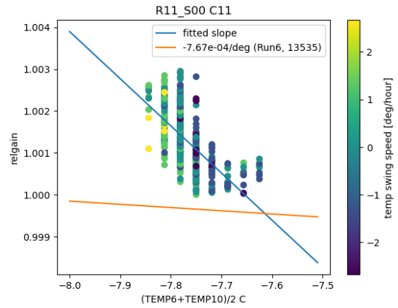
Figure 79: Relative gain as a function of REB temp (TEMP6 and TEMP10), with color based on temperature swing run E1496
