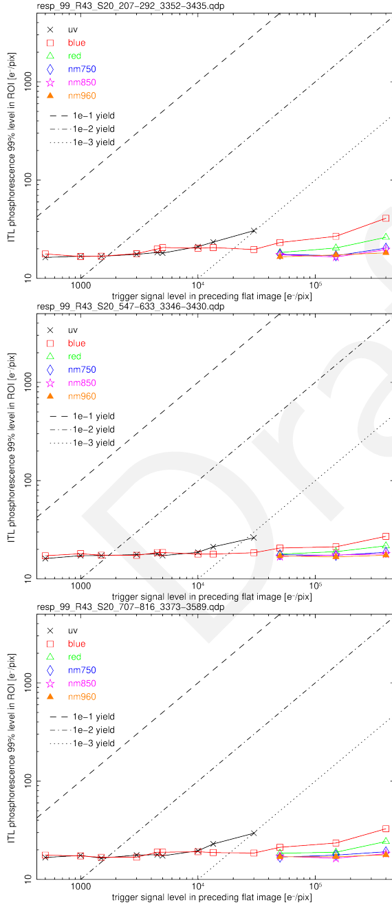
Figure 132: Signal and wavelength response for phosphorescence expression (99% level) in ROIs of images for R43_S20. These include some of the the highly structured snowflake-like transient regions seen in Figs. 98h and 117.
