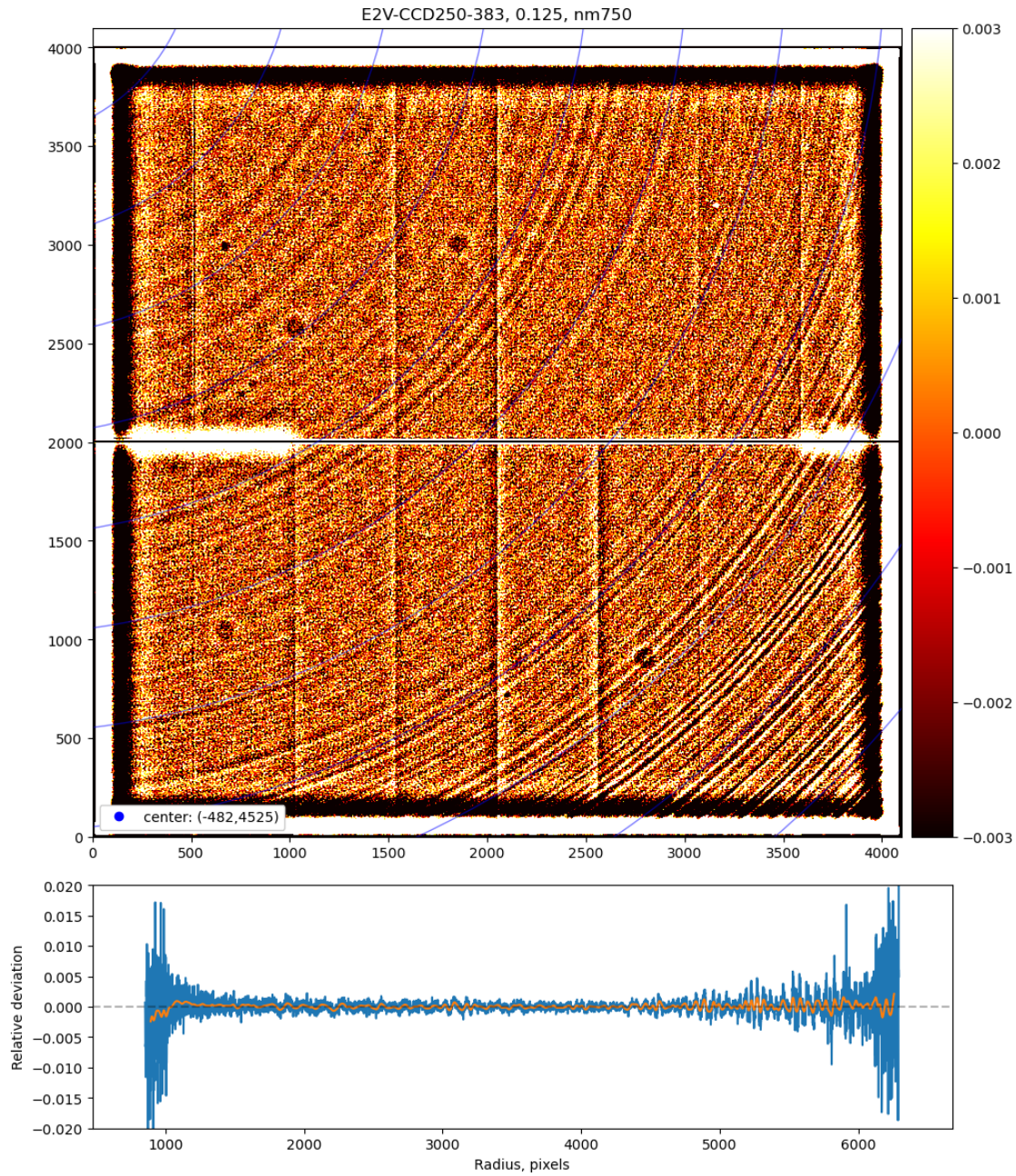
Figure 90: Tree ring with diffuser
