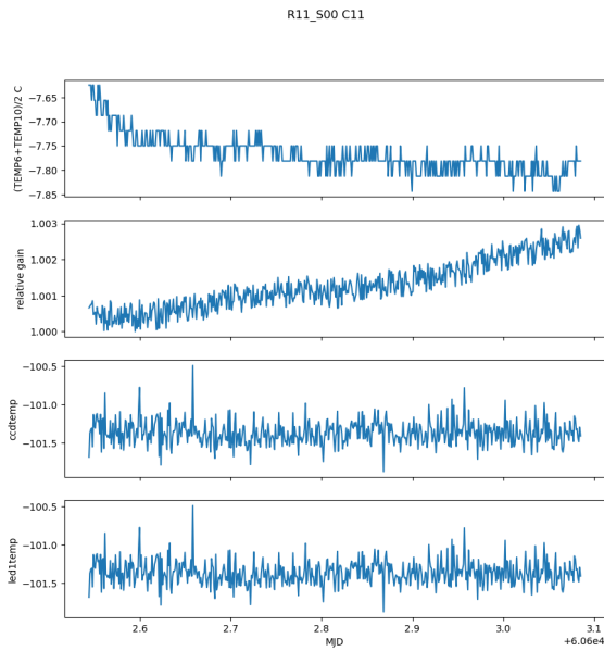
Figure 78: relative gain changes with other parameters for one amplifier R01/S00/C11 in run E1496
