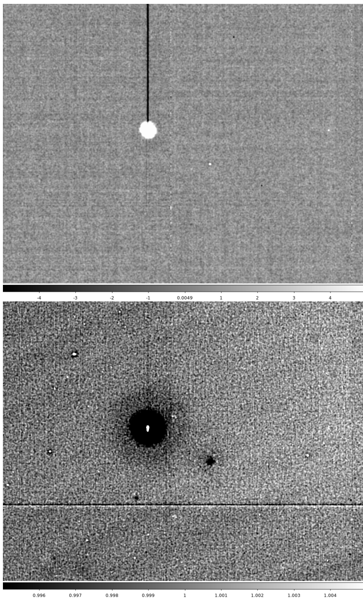
Figure 115: The ITL sensor R03_S10, detail of the vampire pixel of R03_S10_C15. Top: the transient phosphorescence term. Bottom: the blue flat response. As in previous examples, this vampire pixel's transient term is large enough to contaminate the parallel overscan even after the first 15 s following trigger.
