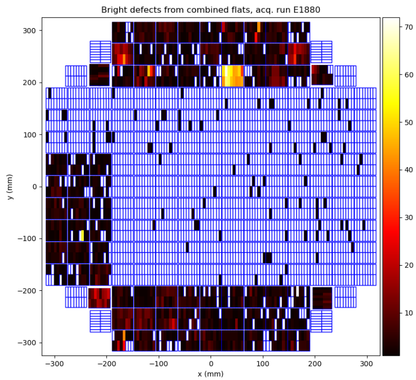
Figure 95: Results of the eo_pipe task written to search for bright defects in combined flats. Using a threshold of 1.2 (120% of flat level), the findings highlights the 8 RTMs that operate ITL sensors (as well as those CRTMs with sensors operating in science mode).
