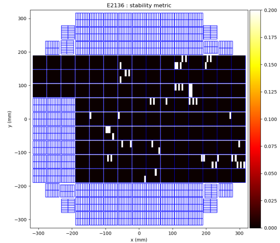
Figure 77: Mosaic of e2v amplifiers identified as unstable (white color) in run E2136
