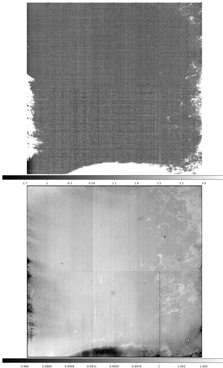
Figure 116: The ITL sensor R43_S11. Top: the transient phosphorescence term. Bottom: the blue flat response. This sensor appears to have the largest integrated phosphorescence among ITL sensors studied. The flat response feature has opposite polarity from the phosphorescence.
