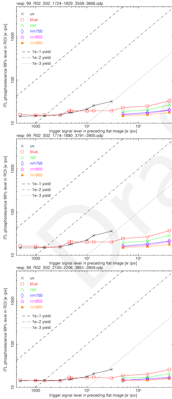
Figure 127: Signal and wavelength response for phosphorescence expression (99% level) in ROIs of images for R02_S02. This is the diffuse phosphorescence that correlates with the coffee stains seen in Fig. 113. No extractions were performed on the vampire pixels found on the same sensor (R02_S02_C15 and R02_S02_C07).
