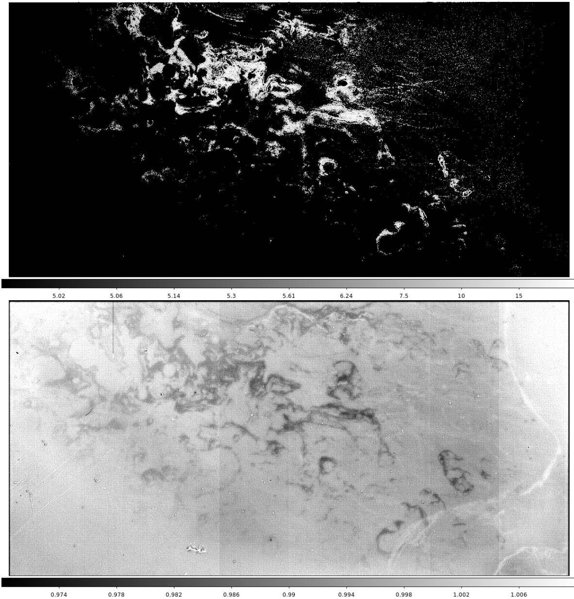
Figure 96: R00_SW1 image showing phosphorescence (top) with morphology similar to the “coffee stains” (bottom) observed with blue CCOB LED illumination. The phosphorescence acquired in dark exposures within the first 15 s following trigger (top) uses a logarithmic stretch with limits 5–25 e^- /pixel. The blue flat field (bottom) is displayed normalized, with 4% stretch limits (0.97 to 1.01), for a target signal level of 10^4 e^- /pixel. Note that the phosphorescence pattern resembles the dark wisps in the flat (with opposite polarity) but that there are apparently no significant phosphorescence features corresponding to the bright wisps.
