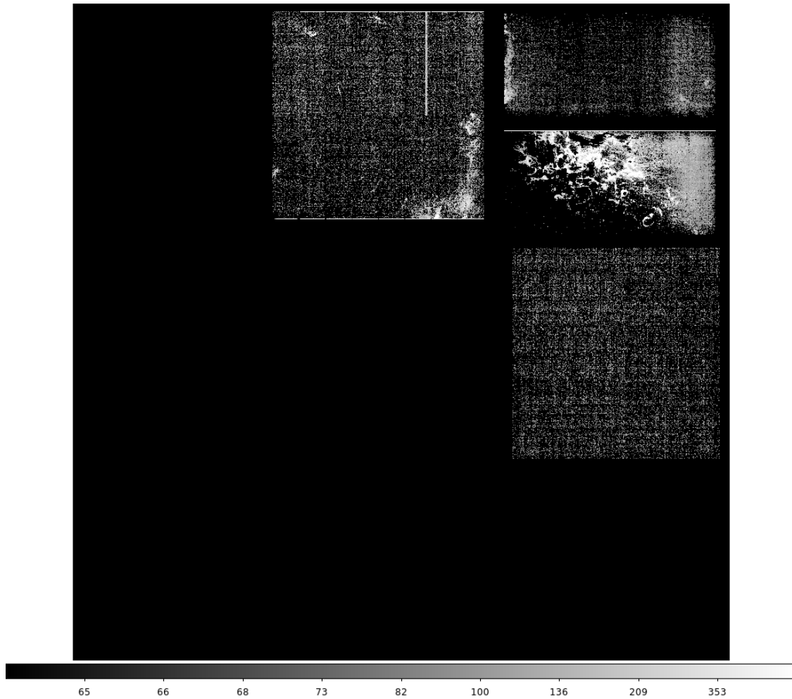
Figure 100: Phosphorescence transients for the R00 CRTM captured in the first 15 s following red CCOB LED at 400 \text{ ke}^-/\text{pix} . With 8 \times 8 blocking, the upper end of the color scale (640) corresponds to 10 \text{ e}^-/\text{pixel} when averaged over 64 pixels contributing.
