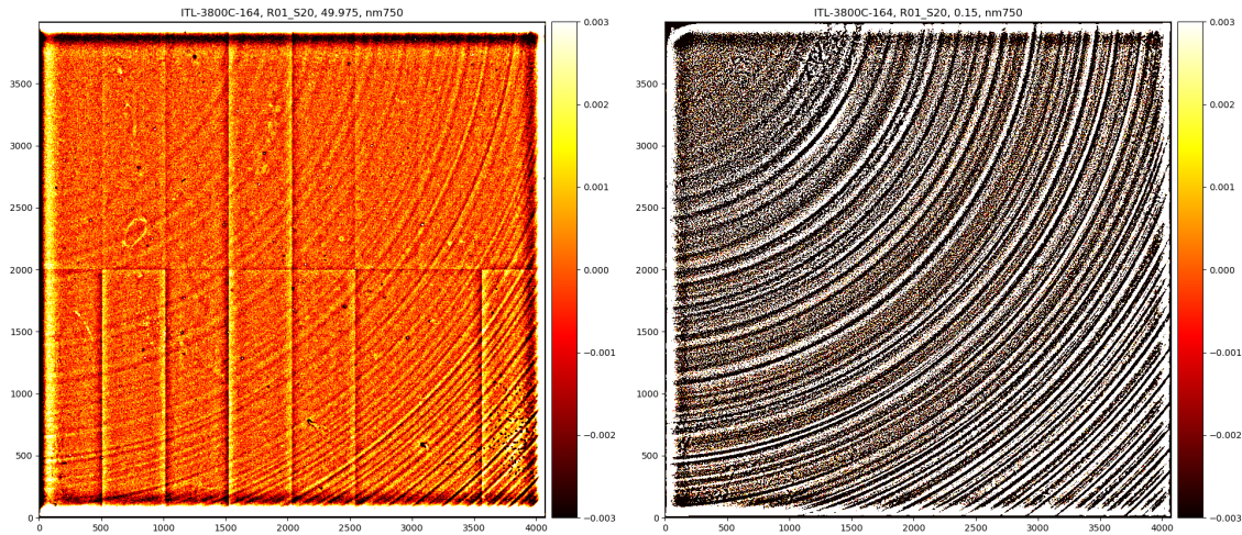
Figure 91: Comparing Tree Rings pattern on the sensor R01_S20 with (left) and without (right) back bias voltage (50 V), we can clearly see that back bias voltage reduces the impact of the tree ring effect.
