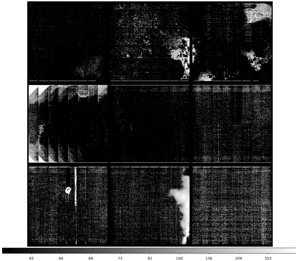
Figure 101: Phosphorescence transients for the R01 RTM captured in the first 15 s following red CCOB LED at 400 \text{ ke}^-/\text{pix} . With 8 \times 8 blocking, the upper end of the color scale (640) corresponds to 10 \text{ e}^-/\text{pixel} when averaged over 64 pixels contributing.
