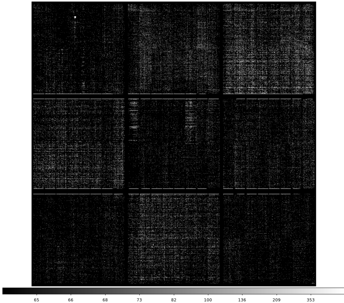
Figure 106: Phosphorescence transients for the R20 RTM captured in the first 15 s following red CCOB LED at 400 \text{ ke}^-/\text{pix} . With 8 \times 8 blocking, the upper end of the color scale (640) corresponds to 10 \text{ e}^-/\text{pixel} when averaged over 64 pixels contributing.
